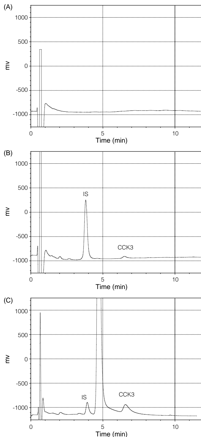
Figure 2. HPLC chromatograms of CCK3 in rat plasma. (A) blank plasma (B) plasma spiked with CCK3 (10 ng/mL) and internal standard (IS) (1 \mu g/mL) (C) rat plasma extracted for 5 min after IV administration of 3.97 mg/kg of CCK3.
