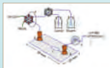
圖二、On-line microfluidics-ICP-MS analytical system. (J. Anal. At. Spectrom., 2013, 28, 1320-1326)
