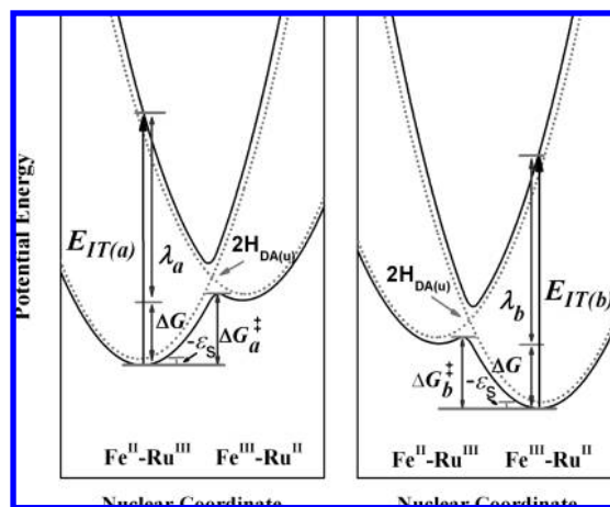
Figure 6. Qualitative illustration of basic parameters in an unsymmetric class II model. The left panel represents the basis for intervalence transfer for [(\text{et-Fcpcy})\text{Ru}(\text{NH}_3)_5]^{3+} and [(\text{et-Fcpcy})\text{Ru}(\text{NH}_3)_4(\text{py})]^{3+} in various solvents, excluding the [(\text{et-Fcpcy})\text{Ru}(\text{NH}_3)_4(\text{py})]^{3+} in nitro-based solvents. Intervalence-transfer behaviors of [(\text{et-Fcpcy})\text{Ru}(\text{NH}_3)_4(\text{py})]^{3+} in nitrobenzene and nitromethane are shown in the right panel. The potential curves for the diabatic limit (dotted curves) and configurational mixing between donor and acceptor states (solid curves) are shown in both panels.
