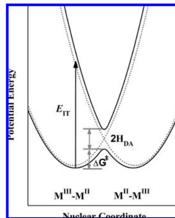
Figure 1. Potential energy curves for the diabatic limit (class I, dotted curve) and the weak coupling (class II, solid curve) in a mixed valence d^5-d^6 ion.
