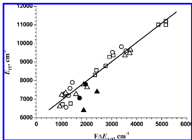
Figure 5. The E_{IT} vs F\Delta E_{1/2} in various solvents for [(\text{et-Fcpcy})\text{Ru}(\text{NH}_3)_5]^{3+} (open square), [(\text{et-Fcpcy})\text{Ru}(\text{NH}_3)_4(\text{py})]^{3+} (open circle), and [(\text{et-Fcpcy})_2\text{Ru}(\text{NH}_3)_4]^{3+} (open triangle). The slope, intercept, and correlation coefficient ( R^2 ) of the least-squares line without the [(\text{et-Fcpcy})\text{Ru}(\text{NH}_3)_4(\text{py})]^{3+} and [(\text{et-Fcpcy})_2\text{Ru}(\text{NH}_3)_4]^{3+} in nitromethane and nitrobenzene (solid circle and triangle) were 1.04 \pm 0.04 , 5900 \pm 120 \text{ cm}^{-1} , and 0.96, respectively.
